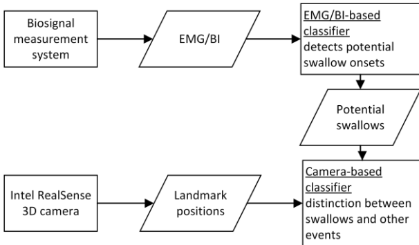
Fig 2. Two-step-classification process.
