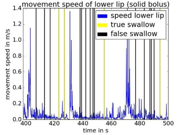
Fig 4. Swallow onsets detected by the EMG/BI-based classifier while swallowing bread.
