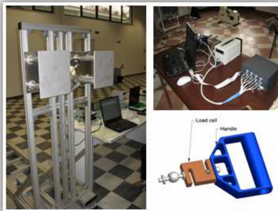
Fig. 1 Pullgrip Dynamometer, Software and Handle with load cell.
