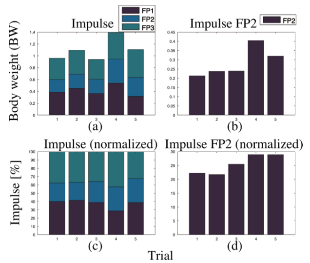
Fig 4. Impulse distribution on the three platforms: 4a. Impulse, 4b. Impulse FP2, 4c. Impulse (normalized), 4d. Impulse FP2 (normalized).
