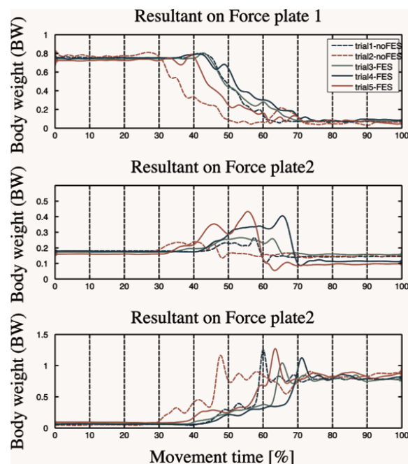
Fig 2. Resultant forces for each trial on both scenarios.
