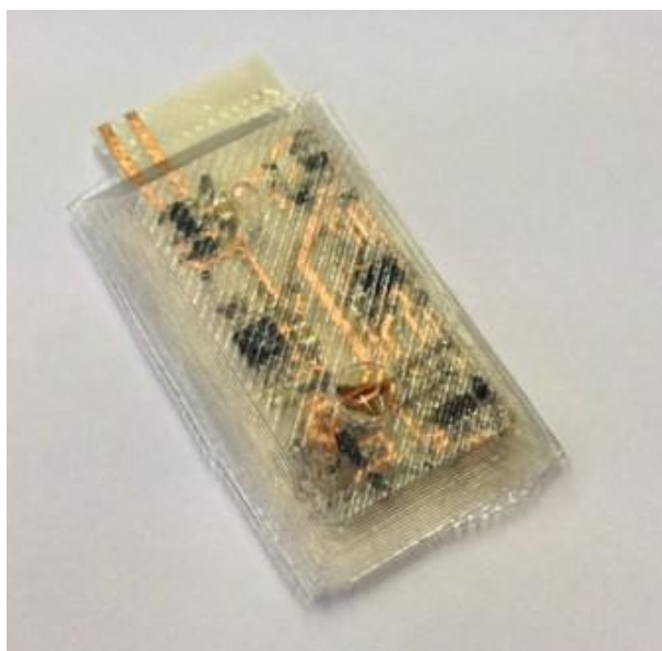
Fig 3. Flexible circuit of our gastro-stimulator encapsulated through vacuum centrifugation
