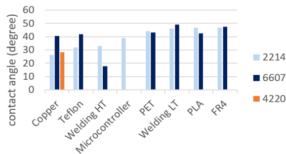
Fig 2. Contact angles of droplets of MED4-4220, MED-6607 and MED-2214 freshly extruded on individual components present in the implant manufacture.
