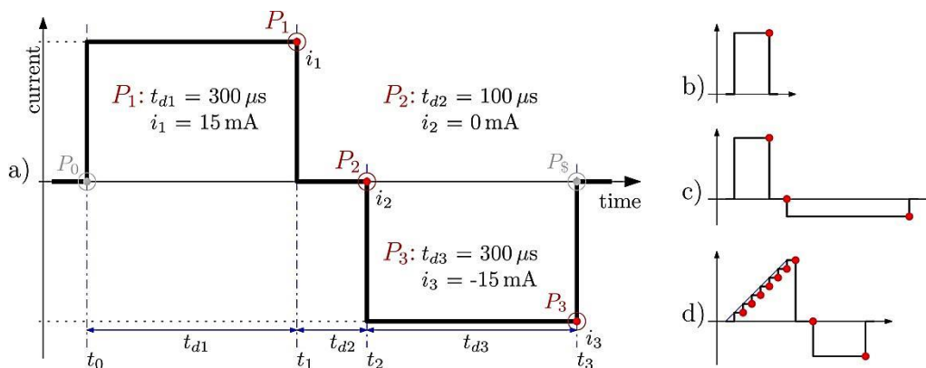
Fig 3. Pulse configuration for a) a standard biphasic pulse, b) a monophasic pulse, c) an unsymmetrical biphasic pulse and d) a custom waveform.
