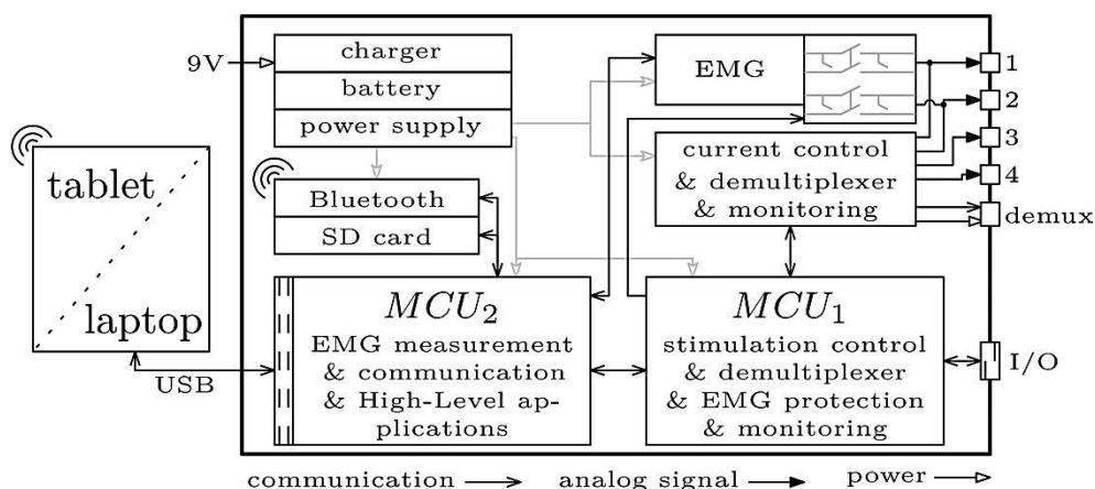
Fig 2. Overview of the RehaMovePro stimulator with the main components.
