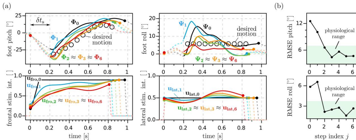
Fig 5. Experimental results from a trial with a chronic drop foot patient. 9 (a) The stimulation intensities are adapted from stride to stride in order to generate the desired foot motion during swing phase. Dots mark heel-rise and initial contact of each stride. Starting from conventional high trapezoidal profiles ( u_{fro,0} and u_{lat,0} ), the ILC adjusts the frontal and lateral stimulation intensity trajectories from trial to trial and thereby improves the foot pitch and roll angle trajectories ( \Phi_i and \psi_i ) from stride to stride. (b) Root-mean-square errors of the foot pitch and roll (data from same trial) are quickly reduced to the ranges of natural variance found in healthy subjects walking at similar velocities. Reproduced with the permission of IFAC. © IFAC 2015. The original figure was published in, 9 and can be found using the Digital Object Identifier (DOI) doi:10.1016/j.ifacol.2015.10.158.
