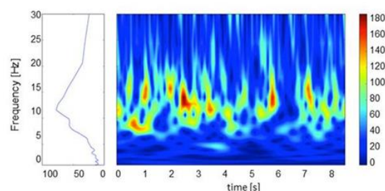
Fig 6. Wavelet spectrum of a realization of an AR(2) process. The process parameters are a_x=0.5 and b_x=-0.5 . It represents a stochastic process which is in good agreement with the wavelet spectra of the MMGs as shown in figure 3.
